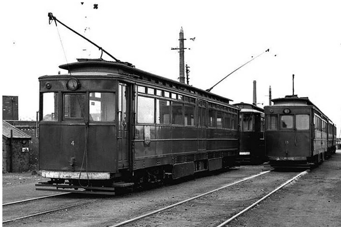
Grimsby & Immingham cars No. 4 one of the original bogie cars; and No. 15 at Immingham. No. 4 dated from 1911 and No. 15 from 1915. No. 4 was the last tram to operate on 1st July 1961. It was 54 feet long and seated up to 72 on wooden seats. (John Kaye).
